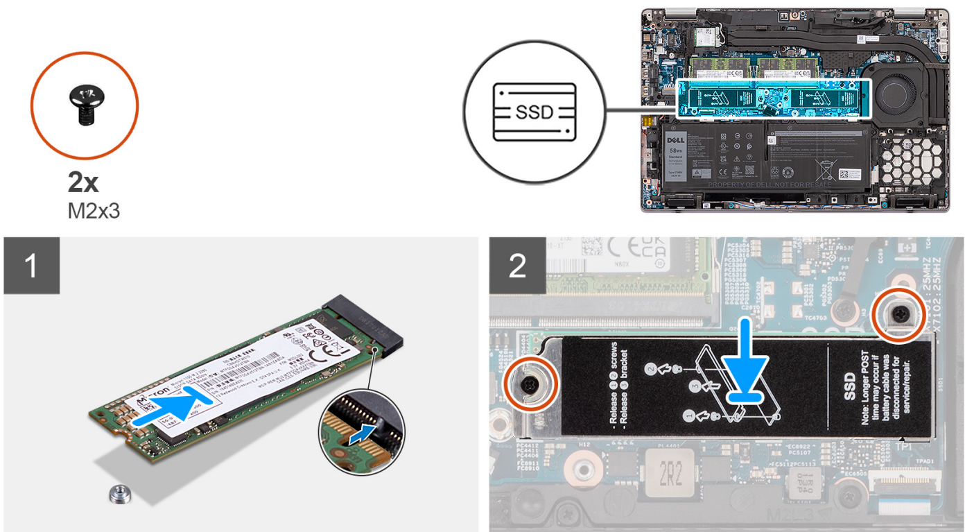
Figure 4. M.2 2280 solid-state drive with bracket
