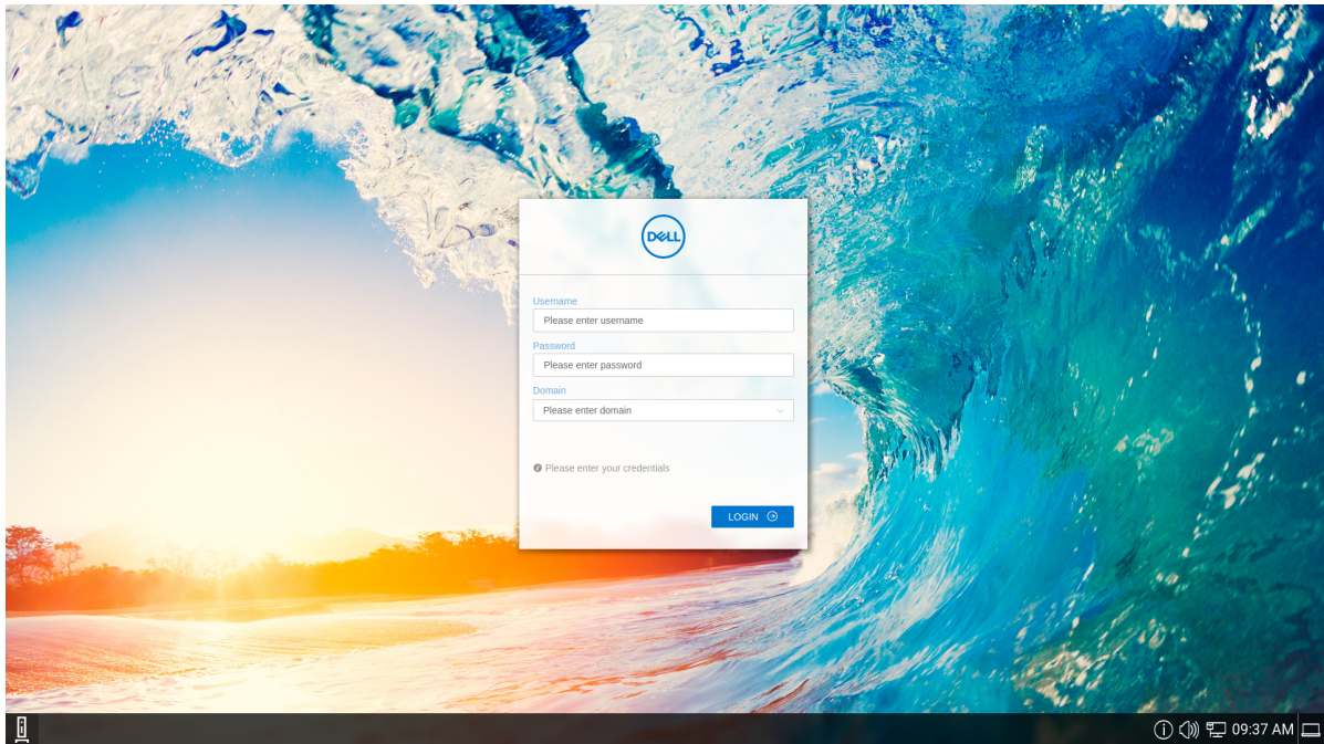
Figure 10. Classic Desktop
