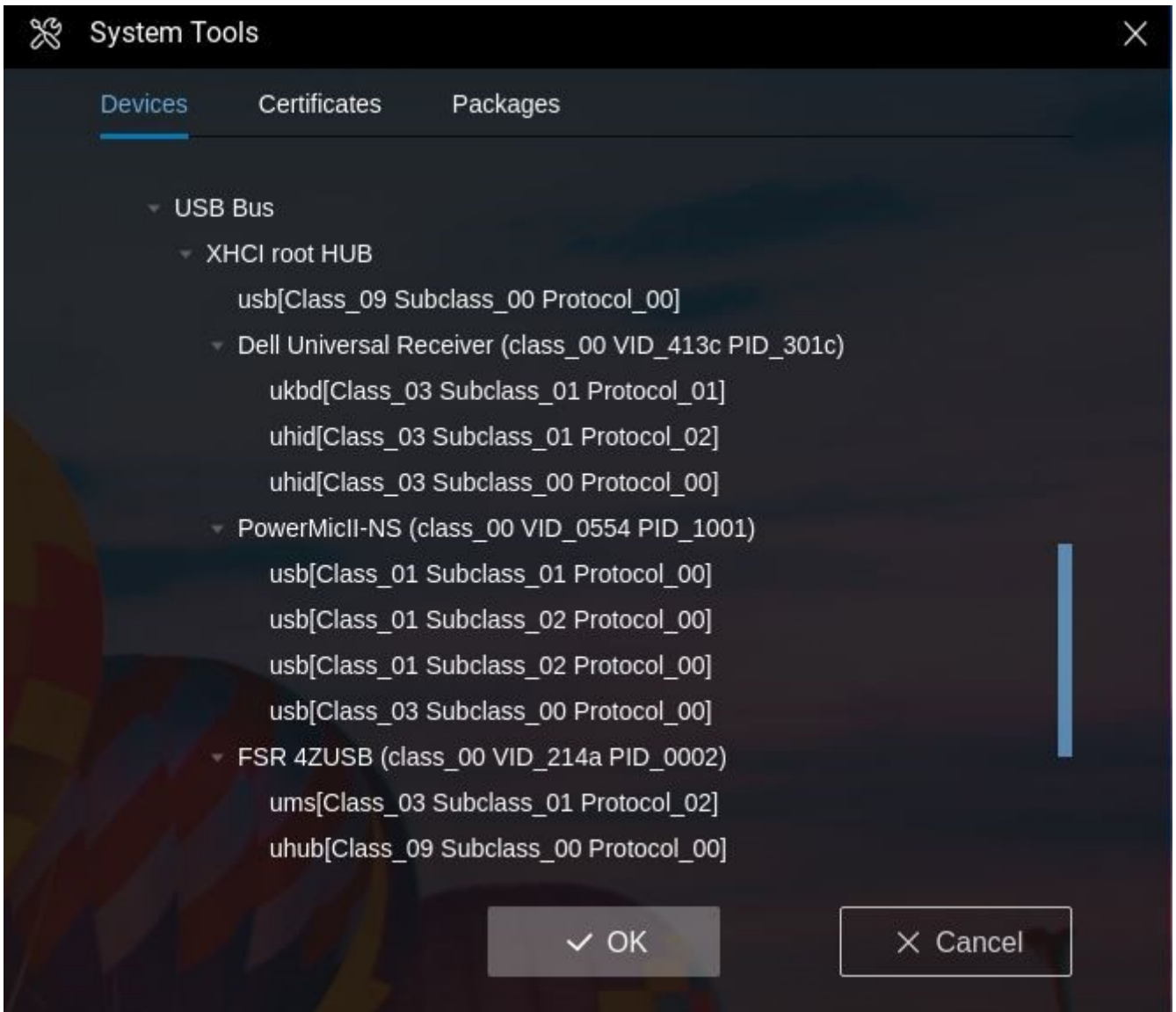
Figure 29. USB redirection
