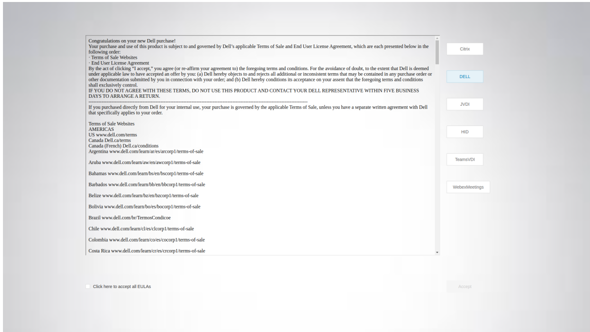
Figure 1. EULA screen
