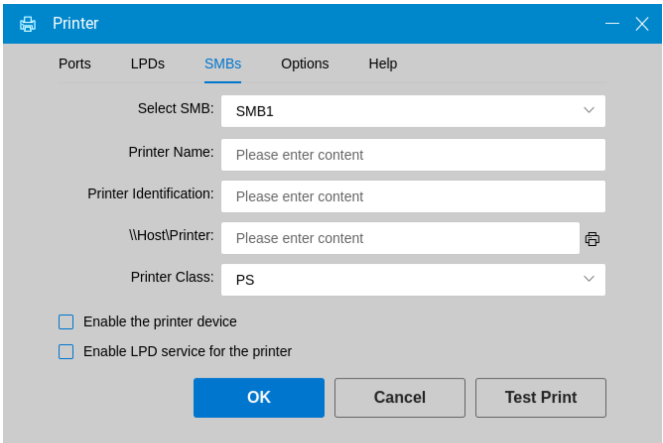
Figure 52. SMB
