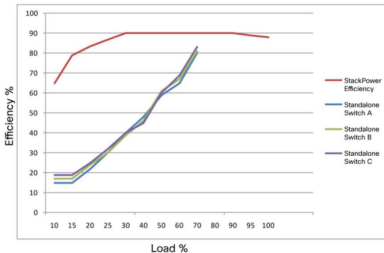
Figure 7. Efficiency Curves
