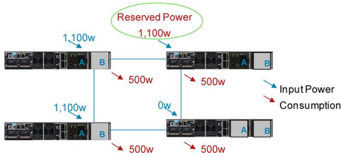
Figure 11. Redundant power
