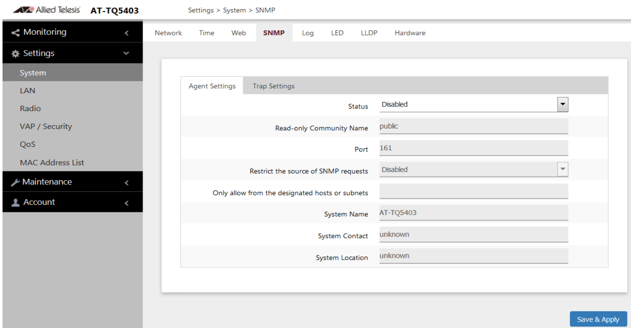
Figure 9. SNMP Agent Settings Window
