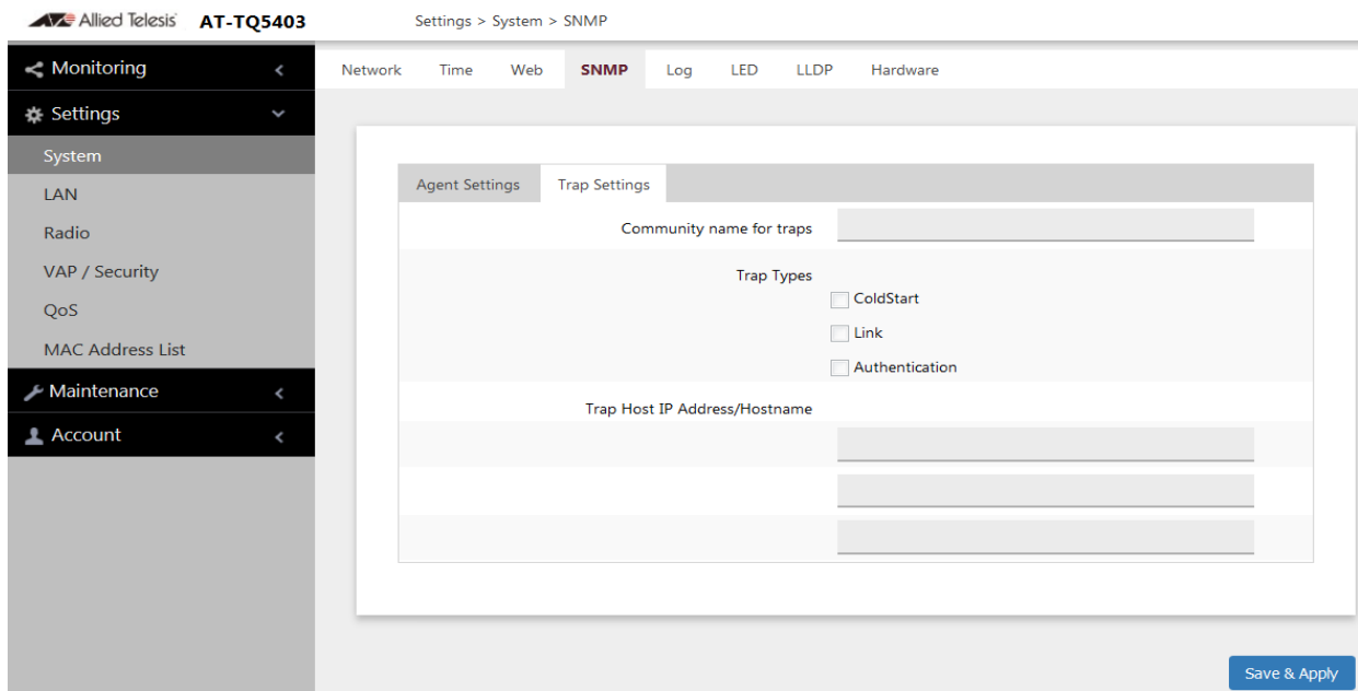
Figure 10. Trap Settings Window
