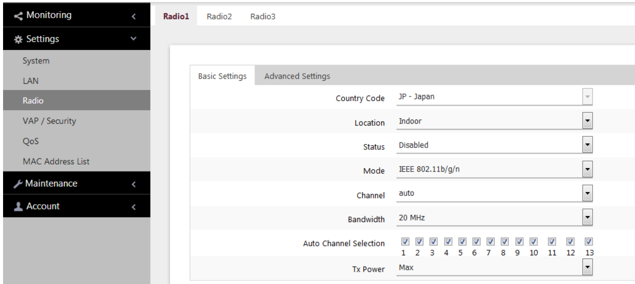
Figure 17. Basic Radio Settings Window on AT-TQ5403e
