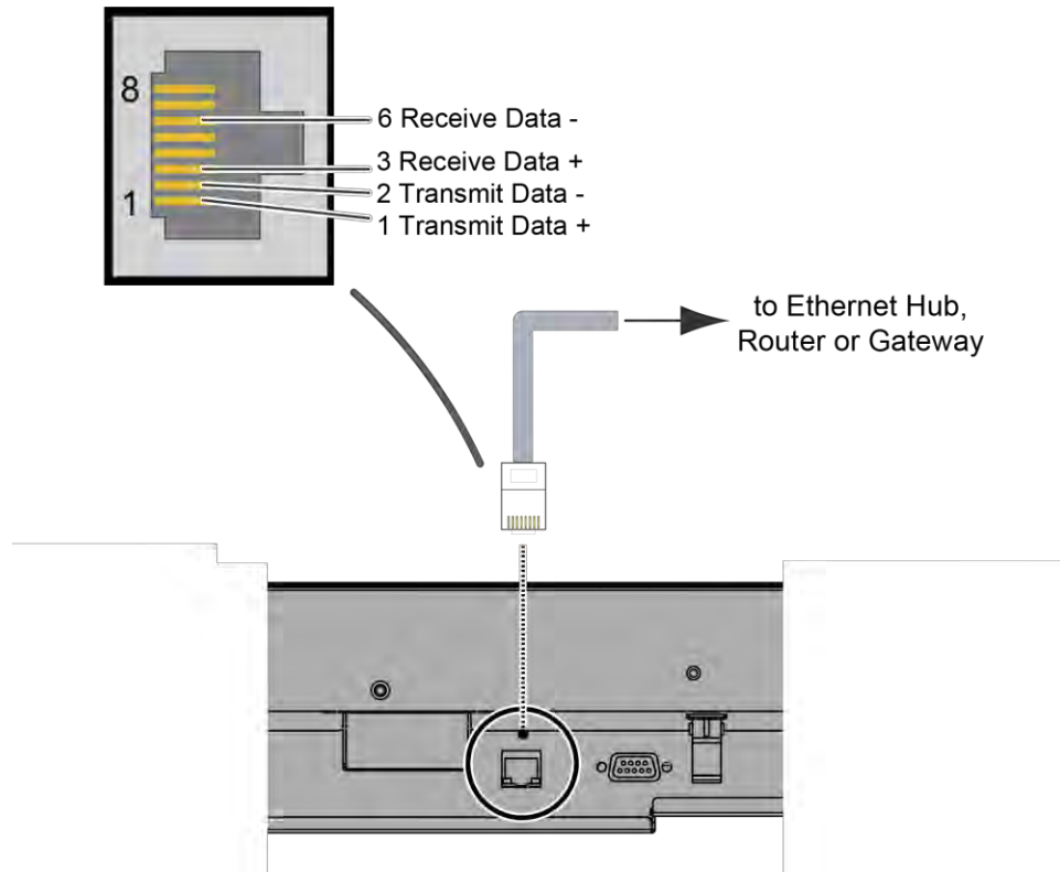
Figure 3-3. Ethernet Connection
