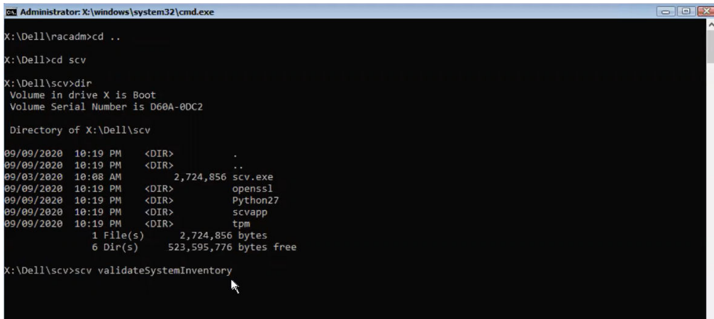
Figure 3. Running the validation command
