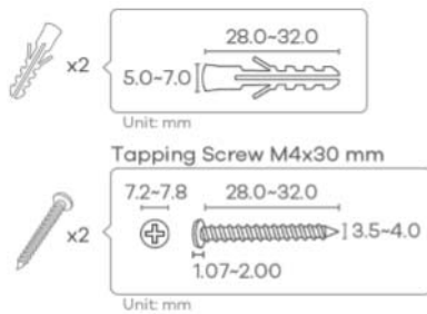
Figure 6 Screw Specifications
