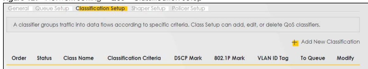
Figure 127 Network Setting > QoS > Classification Setup
