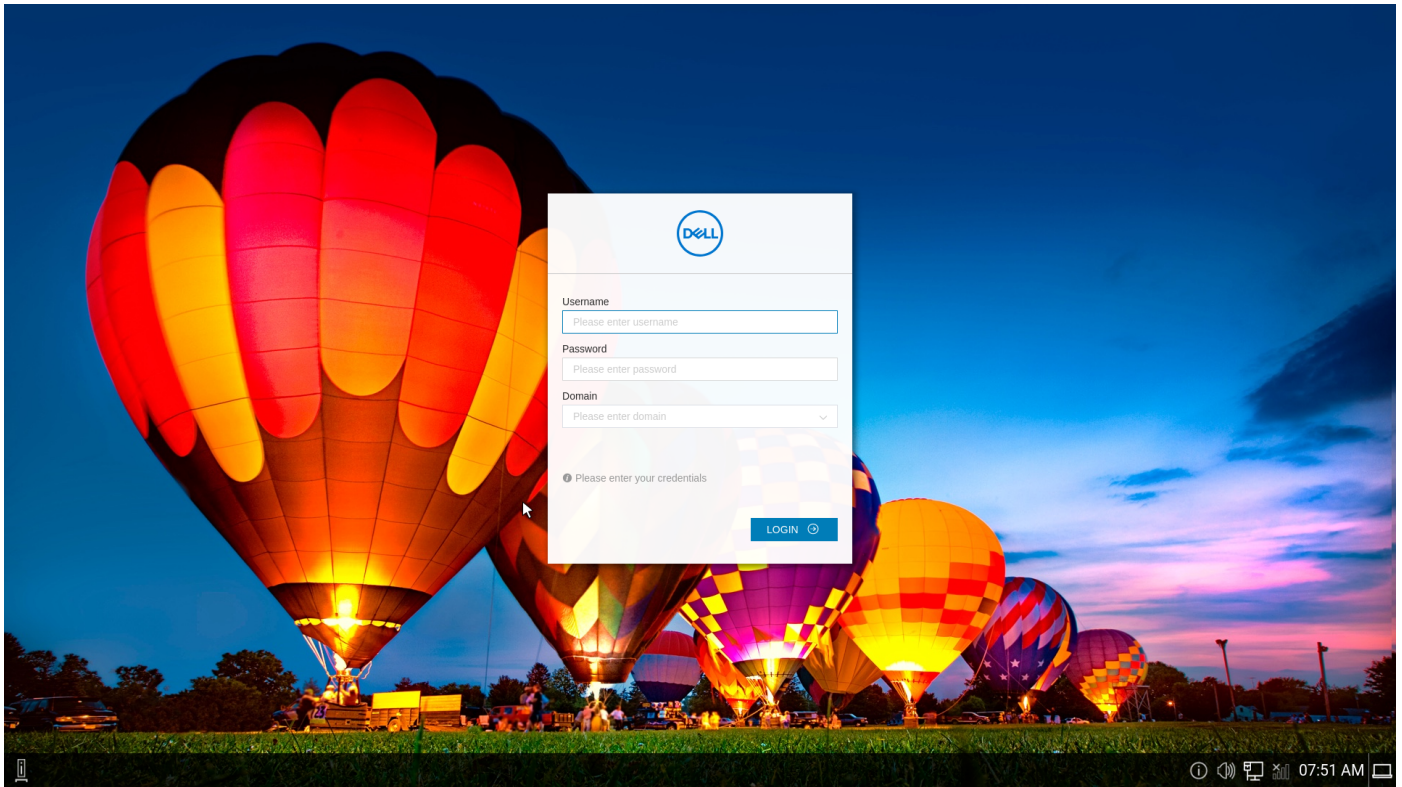
Figure 10. Classic desktop
